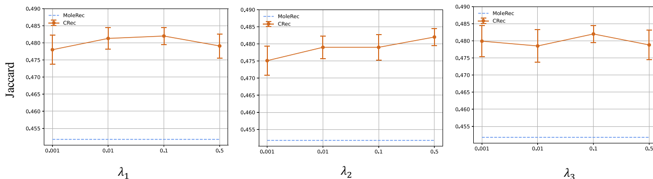
Fig. 4. Hyperparameters sensitivity analysis on the MIMIC-III dataset.
