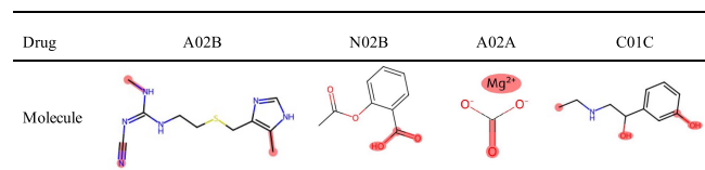
Fig. 3. The visualization of the molecular graphs. (Red highlight: Predicted causal substructure.).
