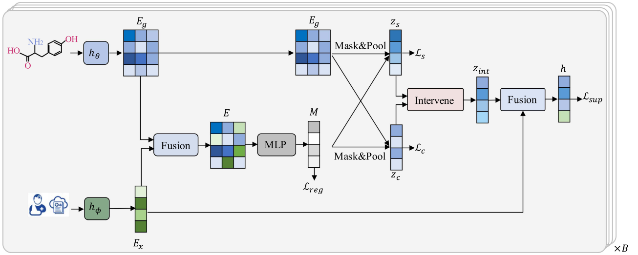
Fig. 2. An overview of CRec. Initially, we encode the input patient data and drug molecular graph to derive their respective representations, denoted as E_x and E_g . Next, we learn the separation mask based on the fused representation E , which combines the patient and molecular representations. Using the learned mask, we separate the original drug molecular representation into causal and spurious parts, represented as z_c and z_s , respectively. Following disentanglement, we employ causal intervention to mitigate the spurious correlation introduced by z_s . Finally, we use the intervened representation to predict the label.
