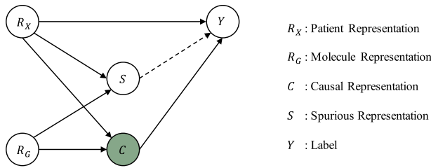
Fig. 1. Structural causal model for the drug recommendation task.
